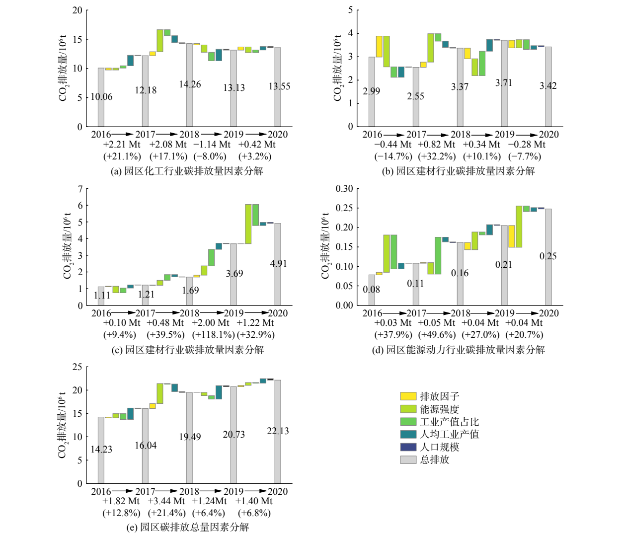
图 3 园区碳排放总量及不同行业类型碳排放量因素分解 Fig. 3 Decomposition analysis of total carbon emissions and carbon emission factors of different industry types in industrial parks
