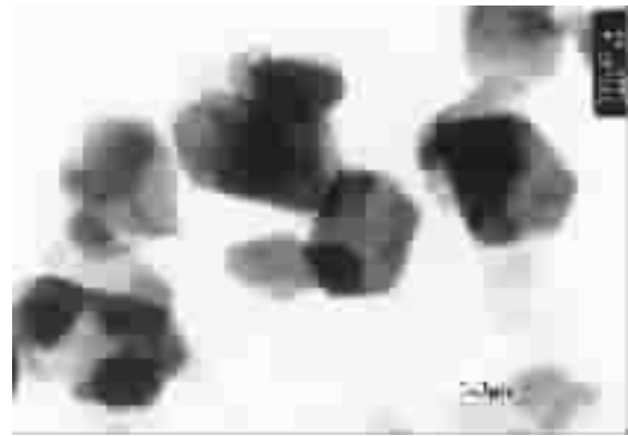
图 4 广西球粘土透射电镜图像 (自生(无序)高岭石呈假六方片状) Fig. 4 TEM image of ball clay (Authigenic (disordered) kaolinite occurs as pseudo-hexagonal flakes)
