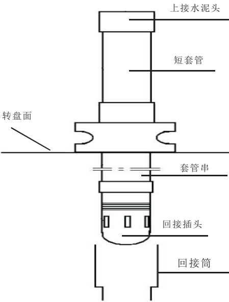
图2 套管短回接工艺示意 Fig.2 Short liner cementing
