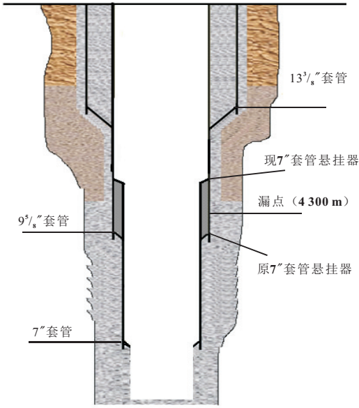
图3 W-8井套管短回接后井身结构 Fig.3 Structure of well W-8 after short liner cementing
