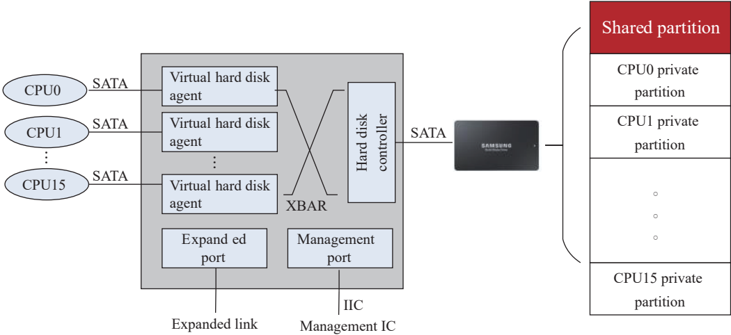
图 8 SATA 硬盘共享架构 Fig.8 Architecture of a SATA disk in shared mode
