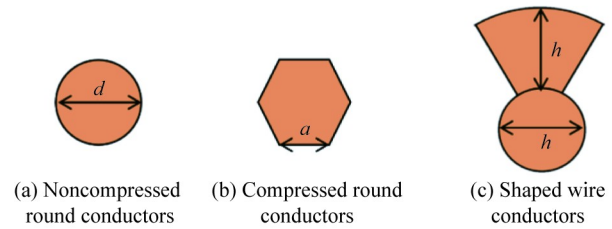
Fig. 5. Simplified shapes of copper wires in conductors of different cross-section types.
