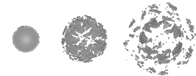
Fig. 5. The fracture behaviour of the base shown at different times (0, 20 and 40 \mu\text{s} ).
