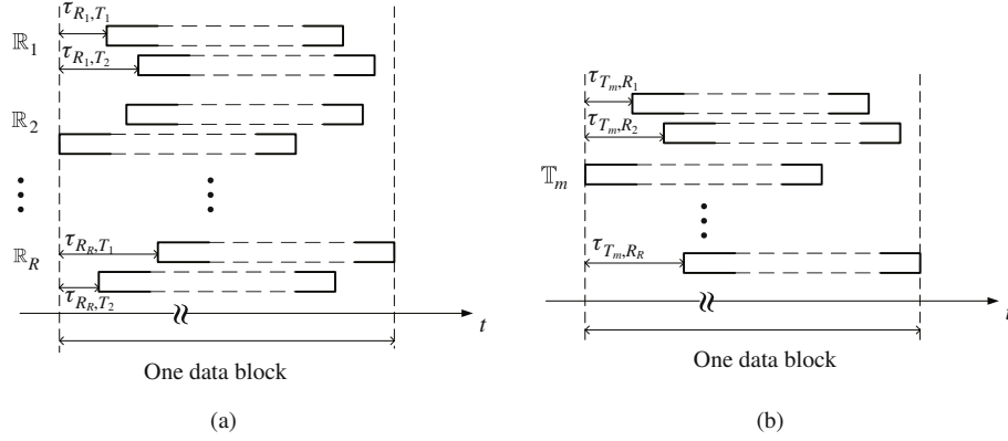
Figure 3 Two kinds of timing errors in a two-way cooperative network [29]. (a) The first kind of timing errors; (b) the second kind of timing errors, where m = 1, 2 .
