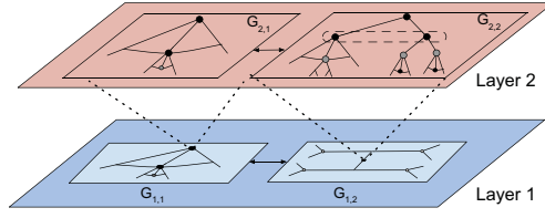
Figure 5. Games-in-games framework for secure and resilient control of multi-layer multi-agent systems. The control of each agent considers the behaviors of the agents at the same layer and the ones at the other layer. Furthermore, the agents also learn and respond to the unanticipated events, such as natural disruptions and adversarial attacks, at each step of decision making.
