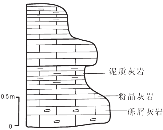
图 4 早—中二叠世地层下部基本层 Fig.4 Essential strata in the lower part of the Early-Mid Permian strata
