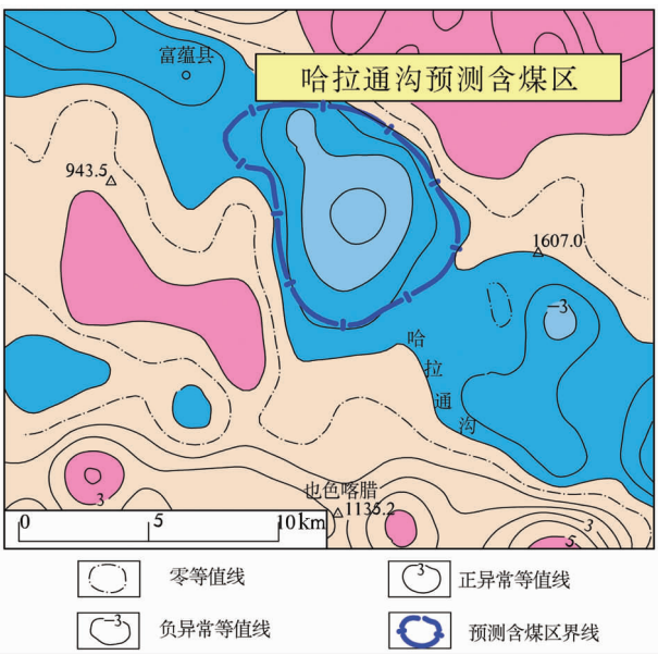
图 3 哈拉通沟预测含煤区剩余重力异常 Fig.3 Residual gravity anomalies of the predicted coal-bearing area in Halatonggou
