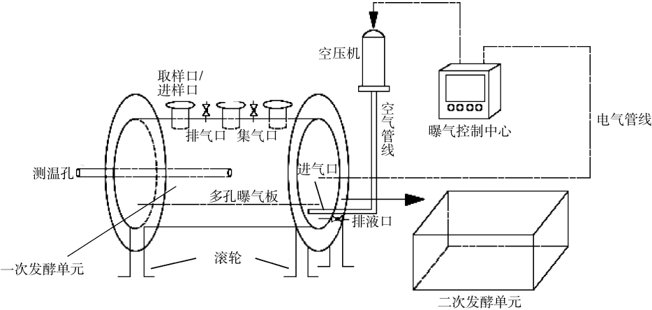
图 1 两段式好氧协同堆肥装置示意图 Fig. 1 Schematic diagram of two-stage aerobic co-composting device
