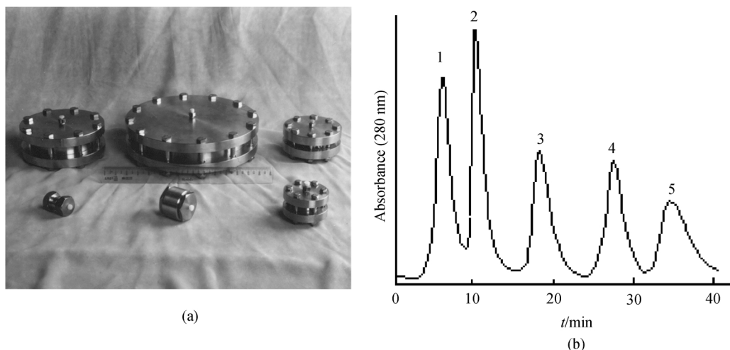
Fig. 1. Photo of the USRPP and chromatogram of five standard proteins. (a) Photo of a set of USRPP in laboratory and preparative scales; (b) chromatogram of five standard proteins separated by the USRPP with 10 \times 200 mm I. D. sample size, 200 \mu L mixture solution containing total proteins 41.5 mg, consisting of cytochrome-C (5.0 mg) (1); myoglobin (7.5 mg) (2); lysozyme (1.5 mg) (3); \alpha -amylase (7.5 mg) (4); insulin (20.0 mg) (5). The linear gradient elution was from 100% solution A [3.0 mol/L ammonium sulphate-0.05 mol/L potassium dihydrogenphosphate (pH 7.0)] to 100% solution B [0.05 mol/L potassium dihydrogenphosphate (pH 7.0)] at a flow rate of 100 mL/min for 40 min with a delay for 10 min. Chart paper speed, 2.5 mm/min; detection wavelength, 280 nm, AUFS: 0.05.
