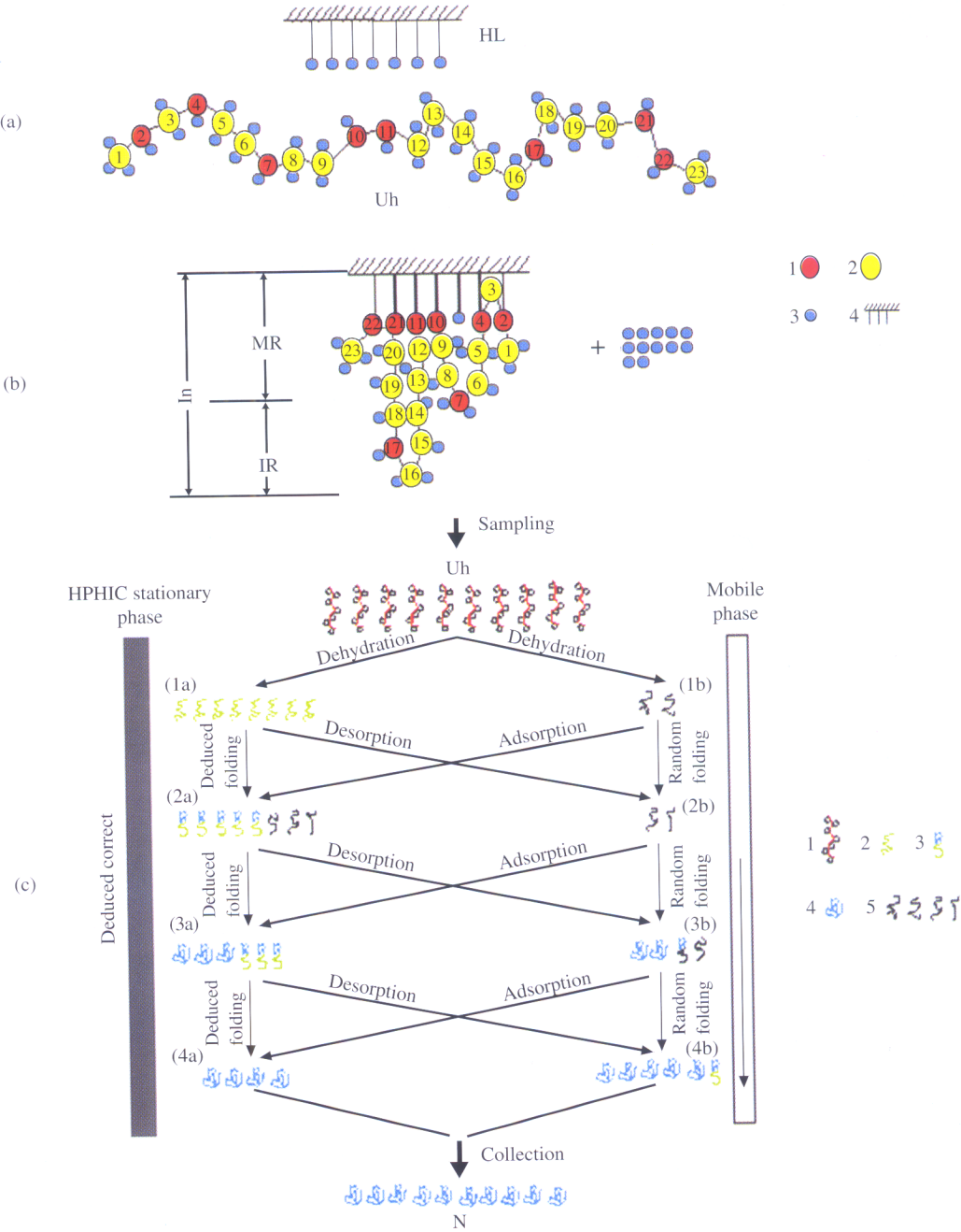
(a) and (b) Schematic model of dehydration and formation of protein intermediates in HPHIC. (a) Hydrated protein and HPHIC stationary phase, (b) formation of intermediate containing microdomain and deduced region. 1, Hydrophobic amino acid residues; 2, hydrophilic amino acid residues; 3, water molecules; 4, ligands of HPHIC stationary phase brush. HL, Hydrated ligands; Uh, unfolded hydrated-amino acid sequence; MR, microdomain region; IR, induced region; In, intermediate. (c) Schematic model of steps for the association between HPHIC stationary and mobile phases for proteins refolding. a, Refolding on the STHIC; b, random refolding in mobile phase. 1a and 1b, Dehydrated unfold protein molecules in adsorbed and desorbed states, respectively; 2a, correct (blue and green colors) and incorrect (black color) intermediates formed on STHIC; 2b, intermediates formed in solution with random folding; 3a, native protein (blue color) and correct intermediates (blue and green colors) on the STHIC; 3b, native protein refolding in mobile phase (blue color) and correct intermediates (blue and black colors), and wrong intermediates (black color); 4a and 4b, protein completely refolding on the STHIC and in the mobile phase, respectively. 1, Hydrated-unfold protein; 2, dehydrated-unfold protein; 3, intermediates containing correct microdomains and deduced structures; 4, correctly refolded protein; 5, wrong folded intermediates.
