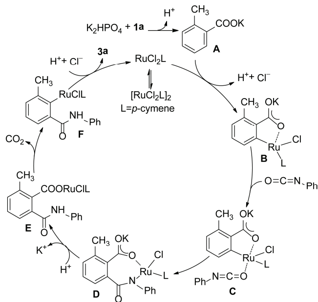
Scheme 2 Proposed catalytic cycle for the ortho -selective decarboxylative C–H amidation of aromatic acids with isocyanates.
