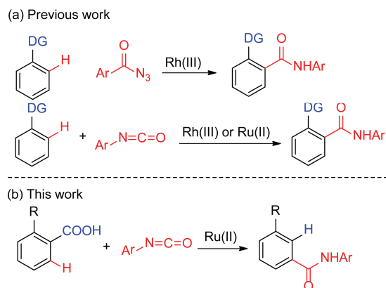
Scheme 1 Synthesis of N -aryl benzamides via C–H functionalization.
