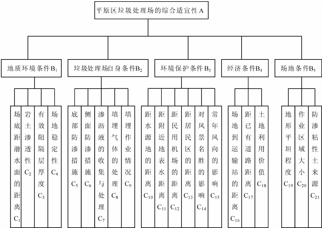
图 1 河北平原区垃圾填埋场适宜性层次结构模型图 Fig.1 Structure model of the suitability hierarchy of the solid waste landfill in Hebei plain area
