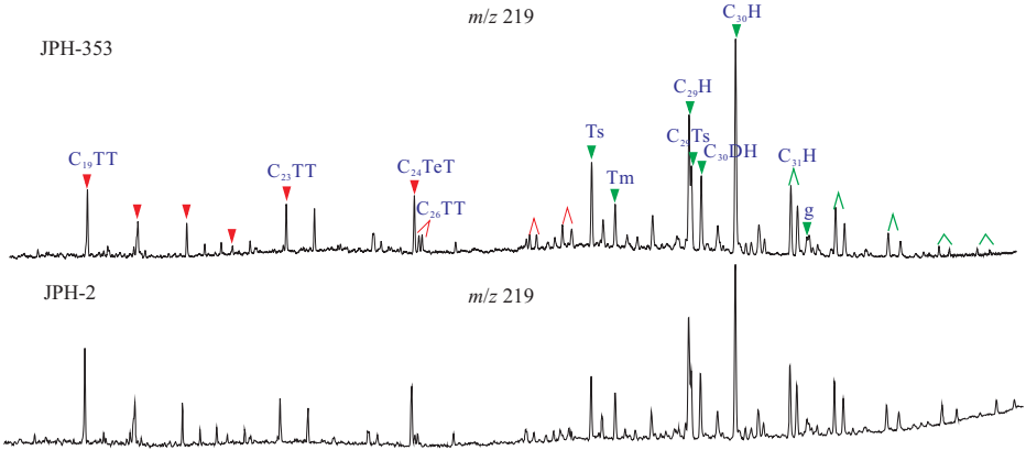
图 4 鄂尔多斯盆地杭锦旗地区上古生界原油萜烷分布特征 Fig.4 Distribution of terpanes in Upper Paleozoic crude oil from Hangjinqi area, Ordos Basin
