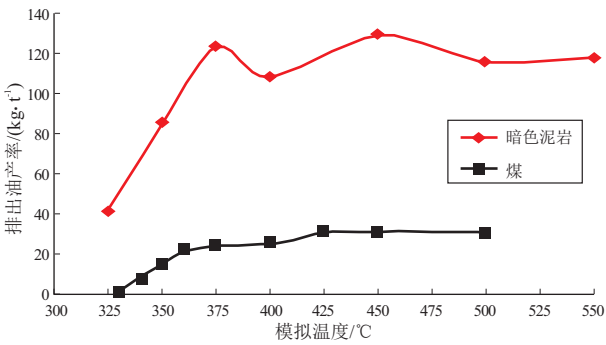
图7 鄂尔多斯盆地杭锦旗地区上古生界煤和暗色泥岩生烃模拟排出油产率曲线 Fig.7 Oil yield curves during hydrocarbon generation simulation on Upper Paleozoic coal and dark mudstone from Hangjinqi area, Ordos Basin
