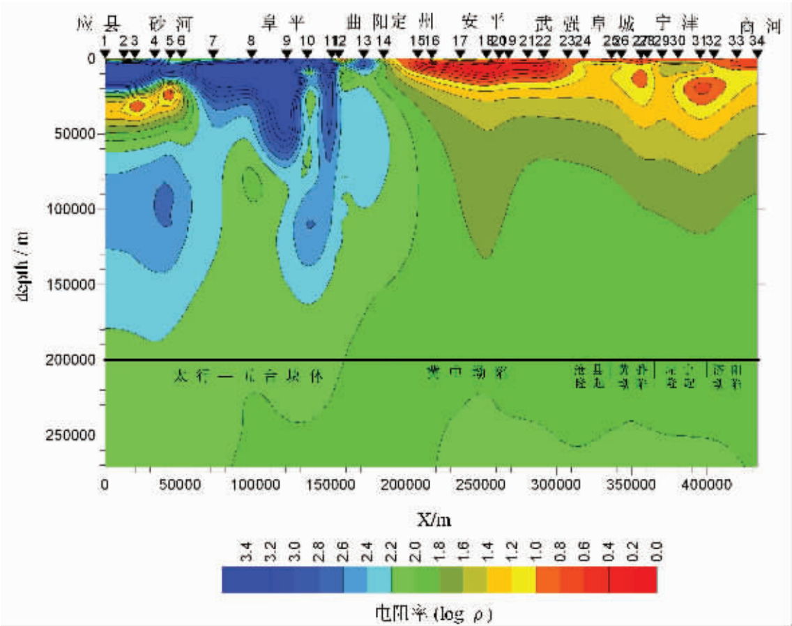
图 3 应县—商河大地电磁二维反演模型 Fig.3 2D model of MT inversion from Yingxian to Shanghe
