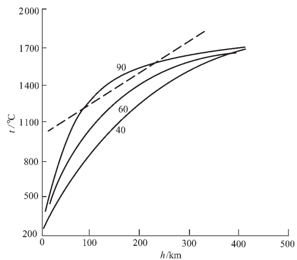
图 4 大陆的地温分布 [1] 虚线为熔化开始时的温度；曲线旁数字为以 \text{mW}/\text{m}^2 为单位的热流量 Fig. 4. Distribution of continental subsurface temperatures [1] The broken line denotes melting temperatures of rock; The numbers beside curves are heat flows (unit: \text{mW}/\text{m}^2 )
