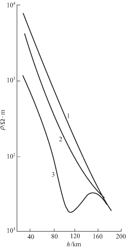
图 1 对于 3 种不同热流量密度得出的大陆电阻率模型 [1] 1—40mW/m 2 ;2—60mW/m 2 ;3—90mW/m 2 Fig.1 Continental resistivity models constructed by using three different heat-flow densities [1] 1—40 mW/m 2 ;2—60 mW/m 2 ;3—90m W/m 2
