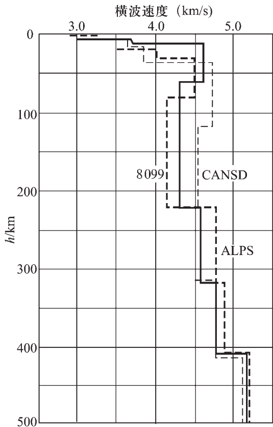
图 6 3 种不同地区壳幔 S 波速度 CANS—加拿大地盾;ALPS—阿尔卑斯; 8099—海洋 Fig.6 S-wave velocities of the crust and mantle in three different kinds of areas [12] CANS—Canada shield; ALPS—Alps; 8099—ocean
