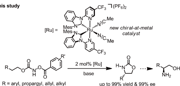
Figure 1 State of the art and this study on asymmetric synthesis of chiral \beta -amino alcohols (color online).
