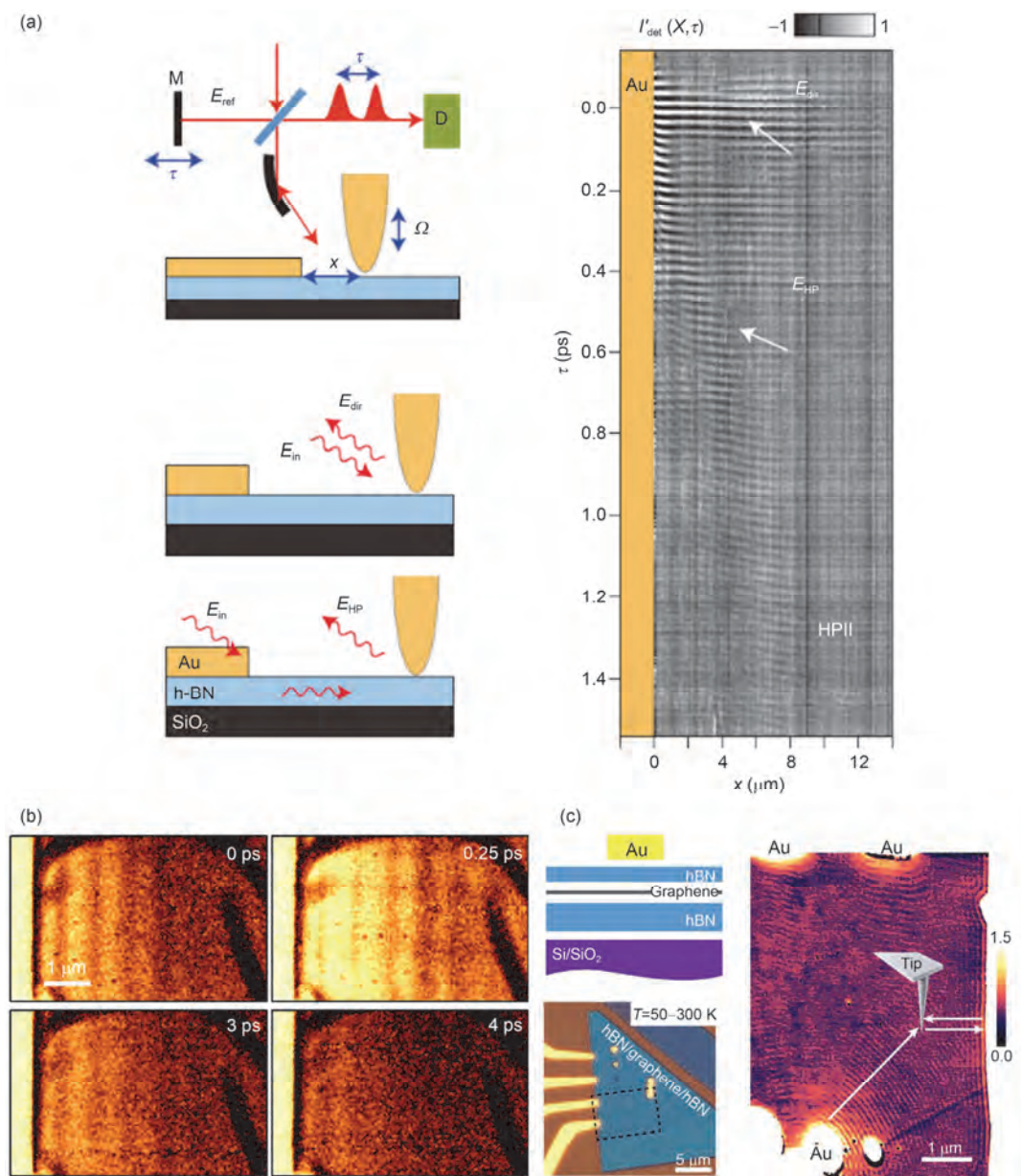
图6 超快及低温s-SNOM对本征电磁模式的成像。(a) 氮化硼声子激元波包成像 [82] ；(b) 黑磷等离激元成像 [83] ；(c) 低温石墨烯等离激元成像 [84] Figure 6 Ultrafast and cryogenic s-SNOM imaging of electromagnetic modes. (a) Imaging of the wave packets of hexagonal boron nitride phonon polaritons [82] . (b) Imaging of black phosphorus plasmon polaritons [83] . (c) Imaging of graphene plasmon polaritons at cryogenic temperatures [84]
