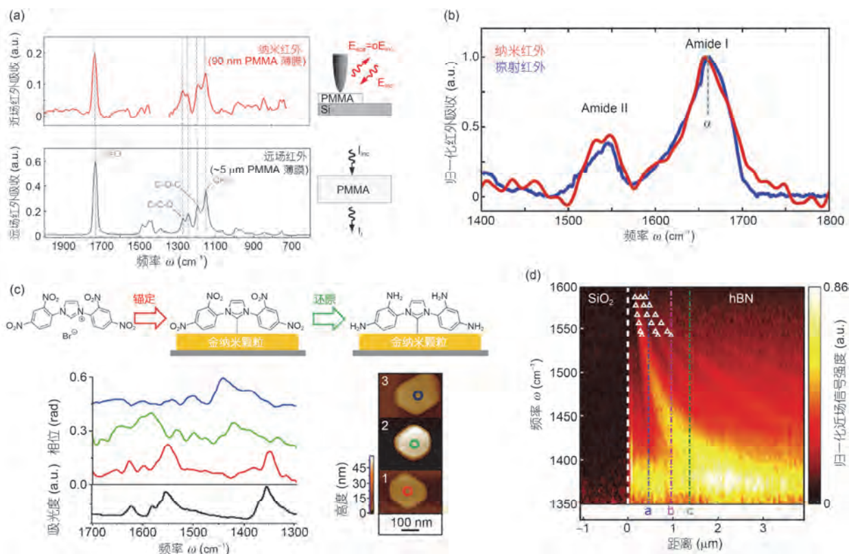
图 7 纳米红外光谱技术 nano-FTIR 的典型应用. (a) 聚甲基丙烯酸甲酯 (PMMA) 近场和远场红外光谱对比 [89] ; (b) 烟草花叶病毒近场和远场红外光谱对比 [90] ; (c) 利用 nano-FTIR 监测金纳米颗粒催化氮杂卡宾还原反应过程 [91] ; (d) 利用 nano-FTIR 获取氮化硼声子激元的频率色散特性 [73] Figure 7 Typical applications of nano-FTIR. (a) Comparison of the near- and far-field infrared spectra of PMMA [89] . (b) Comparison of the near- and far-field infrared spectra of tobacco mosaic virus [90] . (c) Monitoring catalytic reactions on single nanoparticles using nano-FTIR [91] . (d) Mapping dispersions of hexagonal boron nitride phonon polaritons using nano-FTIR [73]
