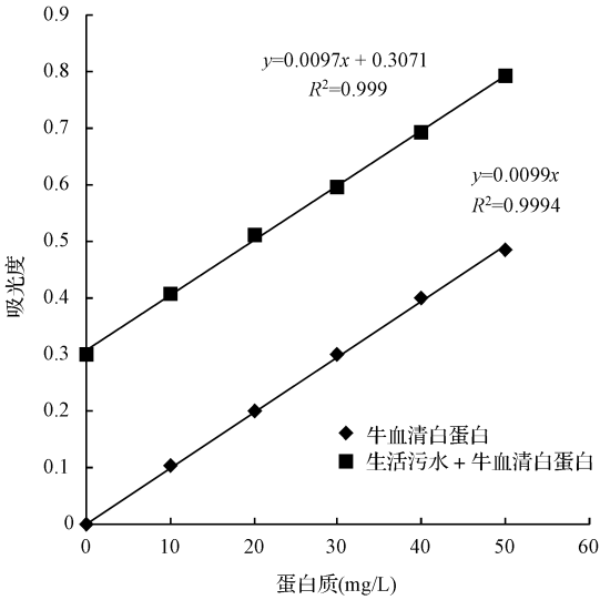
图 2 生活污水对考马斯亮兰染色法测定蛋白质的影响 Fig.2 Effects of domestic wastewater on Bradford method in determining proteins
