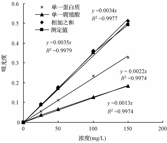
图 1 有腐殖酸存在时蛋白质吸光度变化 Fig.1 Adsorbance changes of proteins while humic acids exist
