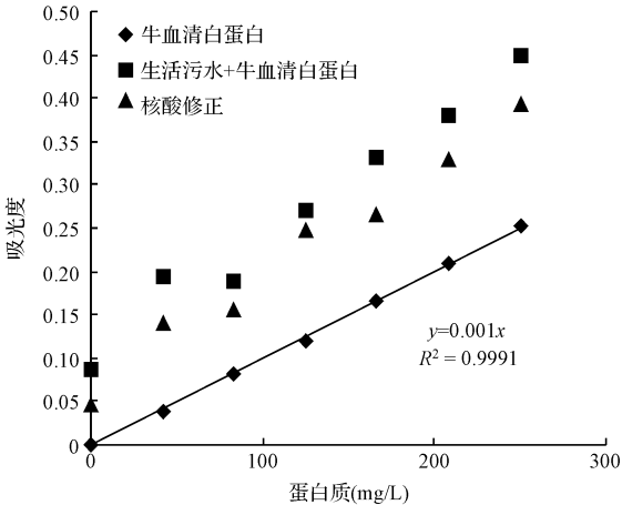
图 3 生活污水对紫外分光光度法测定蛋白质的影响 Fig.3 Effects of domestic wastewater on spectrophotometer method in determining proteins
