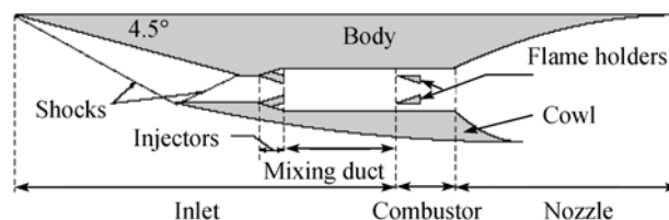
Figure 4 Mixed-compression shcramjet engine [13].
