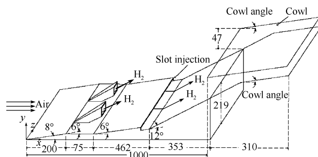
Figure 10 Baseline dual spike scramjet inlet and combustor (unit: mm) [18].
