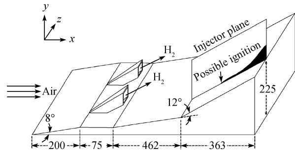
Figure 7 Baseline dual-spike scramjet inlet [7].
