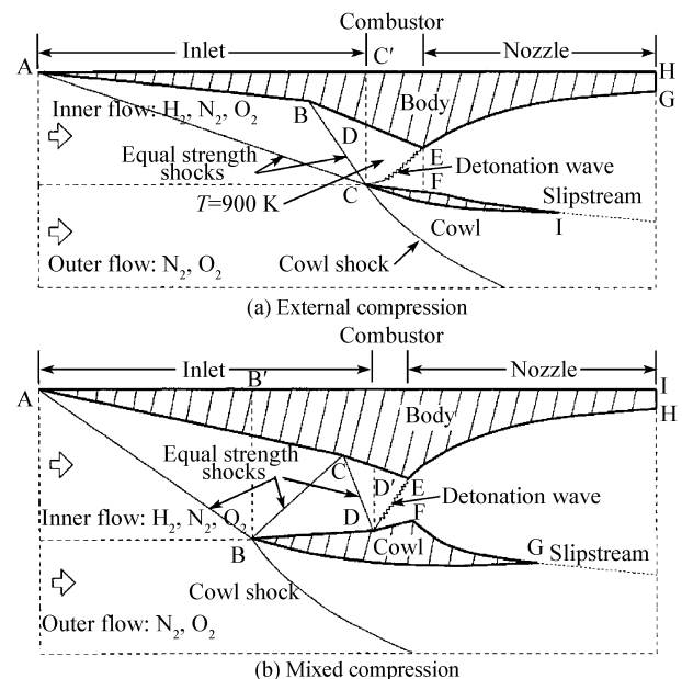
Figure 2 Scramjet model [4].
