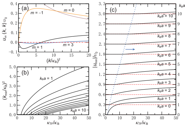
Figure 2 (Color online) Effective e-e interaction u_m . (a) Typical behavior of u_m(k, k) for different m . Parameters: \kappa_B a = 0.2 and \kappa_{\text{TF}}/\kappa_B = 2.6 ; (b) k -position of the u_{m=1}(k, k) minimum as a function of \kappa_{\text{TF}}/\kappa_B for different values of \kappa_B a from 1 to 10; (c) The minimum (most attractive) value of the effective potential for p-wave channel ( m = 1 ) as a function of \kappa_{\text{TF}}/\kappa_B for different values of \kappa_B a . The different curves are offset vertically for clarity, with red dashed lines indicating respective baselines. The dotted line shows the boundary determined from eq. (11) for the onset of attractive interaction. Q_M = 1 .
