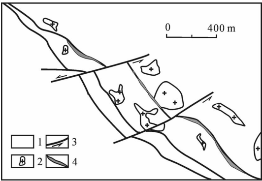
图 7 五龙沟金石灰沟矿段 3 号金矿带地质构造略图 (该矿带在区域构造中的位置见图 2) 1—前寒武纪变质岩; 2—花岗岩类侵入体; 3—断裂; 4—金矿体 Fig.7 Schematic map showing the geology and structure of gold ore zone No. 3 in the Shihuigou ore section of the Wulonggou gold district (for the location of the gold ore zone in the regional structure, see Fig.2) 1—Precambrian metamorphic rocks; 2—Granitoids; 3—Fault (the movement direction shown by arrowhead); 4—Gold orebody
