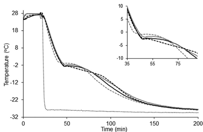
Fig. 2. Cooling curve of gilthead seabream slices: ..... untreated (control) and osmotically pre-treated using different osmotic solutions — HDM, — HDM + treh, — HDM + gluc (..... incubator temperature).
