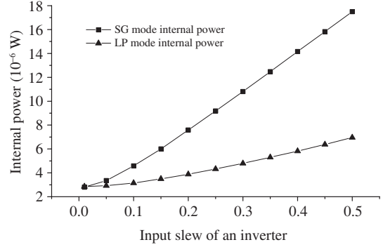
Figure 6 Input slew vs. internal power. Other conditions are as same as Figure 4.
