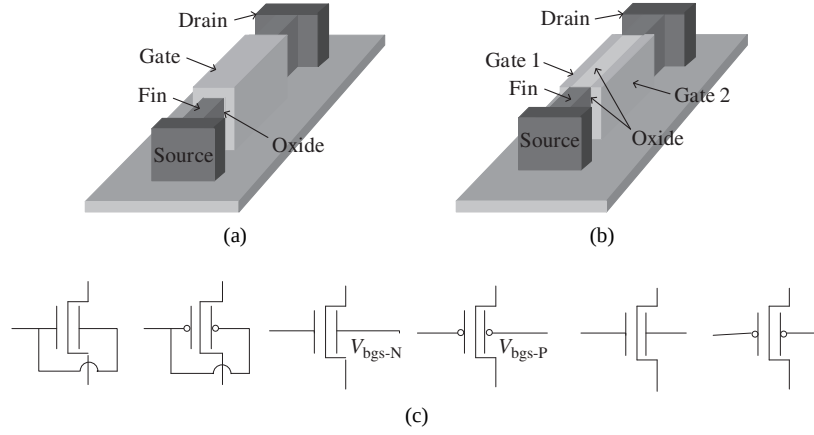
Figure 1 FinFET model and schematics. (a) Tied gate three-dimensional diagram; (b) independent gate three-dimensional diagram; (c) electrical model schematics ( V_{\text{bgs-N}} is Low Bias, V_{\text{bgs-P}} is High Bias).
