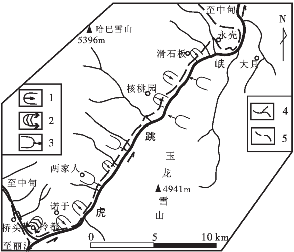
图 8 虎跳峡地区外动力地质灾害分布图 1—滑坡;2—变形体;3—崩塌;4—水系;5—公路 Fig.8 Distribution of geological hazards induced by exogenic forces in the Tiger-Jump Gorge 1-Landslide;2-Deformation mass;3-Rock avalanche; 4-Drainage system;5-Highway
