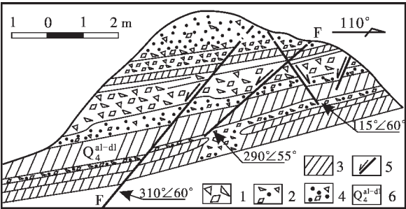
图 3 龙蟠—乔后断裂龙蟠吊桥剖面 1—洪积砾石;2—砂砾层;3—粉砂层;4—含砾砂层; 5—正断层;6—全新世冲洪积物 Fig.3 Section of the Longpan-Qiaohou fault in the Longpan drawbridge on the right bank of the Jinsha River 1-Diluvial gravel;2-Sand and gravel;3-Silt; 4-Gravel-bearing sand;5-Normal fault; 6-Holocene alluvial and diluvial deposits
