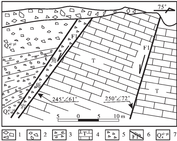
图 2 龙蟠—乔后断裂桥头镇剖面 1—采石弃渣;2—残坡积;3—冲洪积物; 4—三叠纪碎裂灰岩;5—断层角砾岩;6—龙蟠—乔后断裂; 7—全新世混杂堆积物 Fig.2 Section of the Longpa-Qiaohou fault at Qiaotou Town 1-Waste quarry stone;2-Eluvium;3-Alluvial and proluvial deposits;4-Triassic fractured limestone;5-Fault breccia; 6-Longpan-Qiaohou fault;7-Holocene deposits
