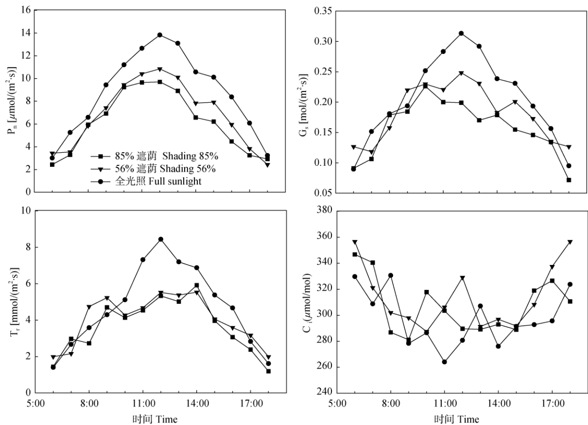
图 1 遮荫处理下梅叶冬青的净光合速率( P_n )、气孔导度( G_s )、蒸腾速率( T_r )和胞间 CO_2 浓度( C_i )的日变化 Fig. 1 Diurnal changes in net photosynthetic rate ( P_n ), stomatal conductance ( G_s ), transpiration rate ( T_r ) and intercellular CO_2 concentration ( C_i ) of Ilex asprella under shading
