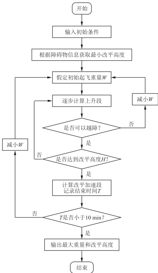
图 4 优化模型算法计算流程图 Fig. 4 Calculation flow chart of optimization model algorithm
