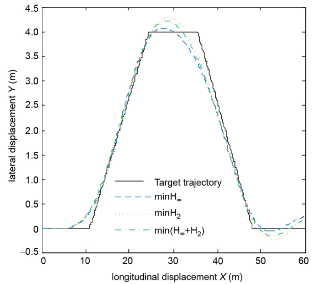
Figure 13 (Color online) Double lane road simulation.
