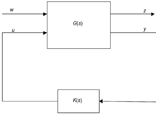
Figure 3 H_\infty standard design problem.
