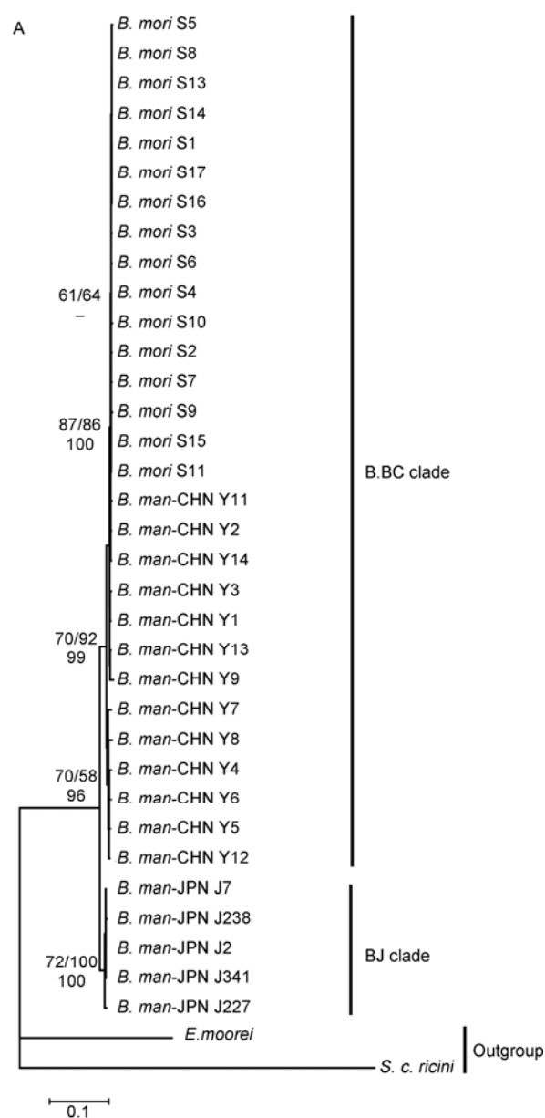
Appendix Figure 1 Bayesian tree based on the TH gene. Support values above the branches represent ML bootstrap (left) and MP bootstrap values, and below the branches represent Bayesian posterior probabilities. “—” indicates bootstrap values or BPP less than 50. B. man -CHN represents the Chinese wild silkworm; B. man -JPN represents the Japanese wild silkworm.
