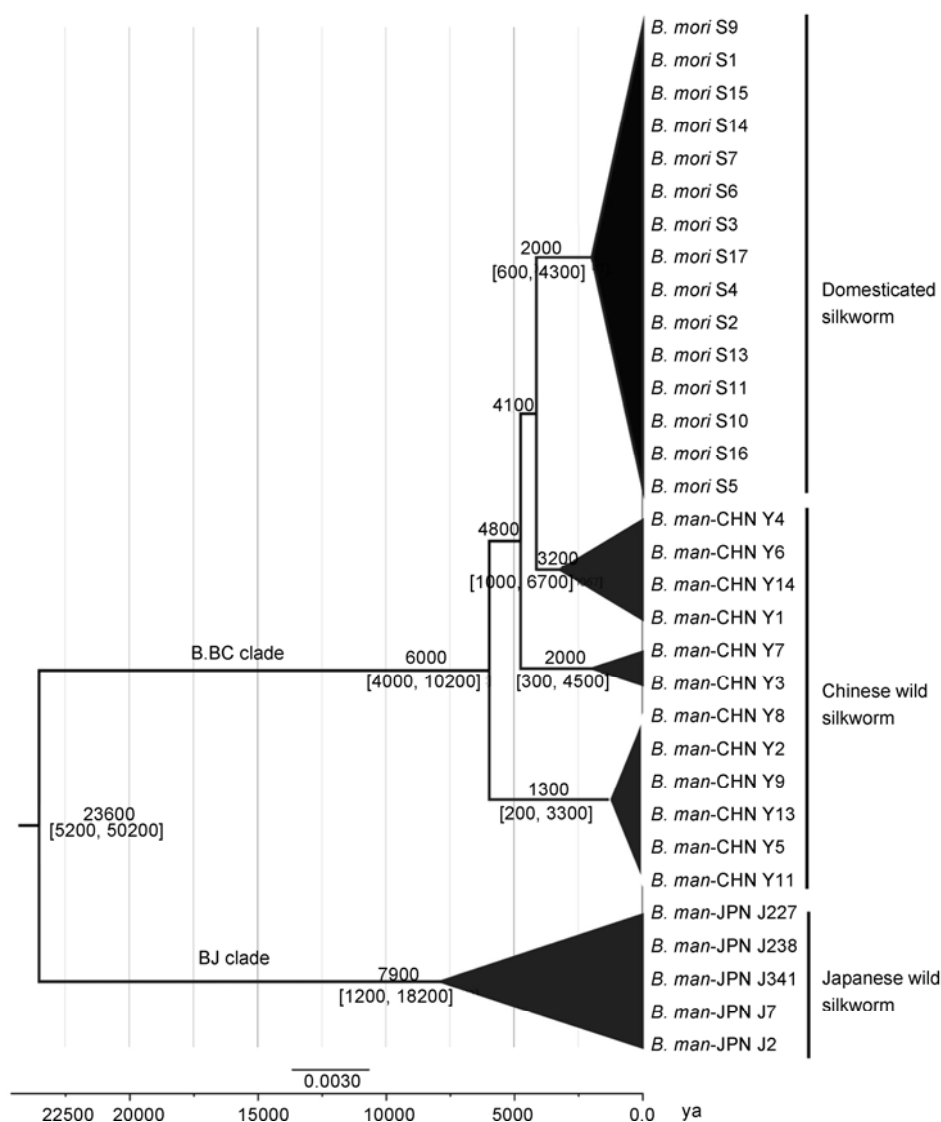
Figure 3 Chronology of divergence times among silkworms based on mtDNA, estimated using Bayesian methods implemented in BEAST. The value above the branch represents the divergence time and below branch is the 95% highest posterior density interval (HPD). B. man-CHN refers to the Chinese wild silkworm; B. man-JPN refers to the Japanese wild silkworm.
