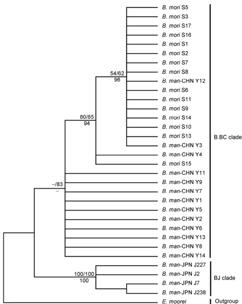
Figure 2 MP Phylogenetic tree reconstruction based on the period gene. Support values above the branches represent ML bootstrap (left) and MP bootstrap values and the values below the branches represent Bayesian posterior probabilities. “-” indicates bootstrap values or BPP less than 50. B. man-CHN is the Chinese wild silkworm; B. man-JPN is the Japanese wild silkworm. E. moorei refers to Ernolatia moorei and S. c. ricini refers to Samia cynthia ricini .
