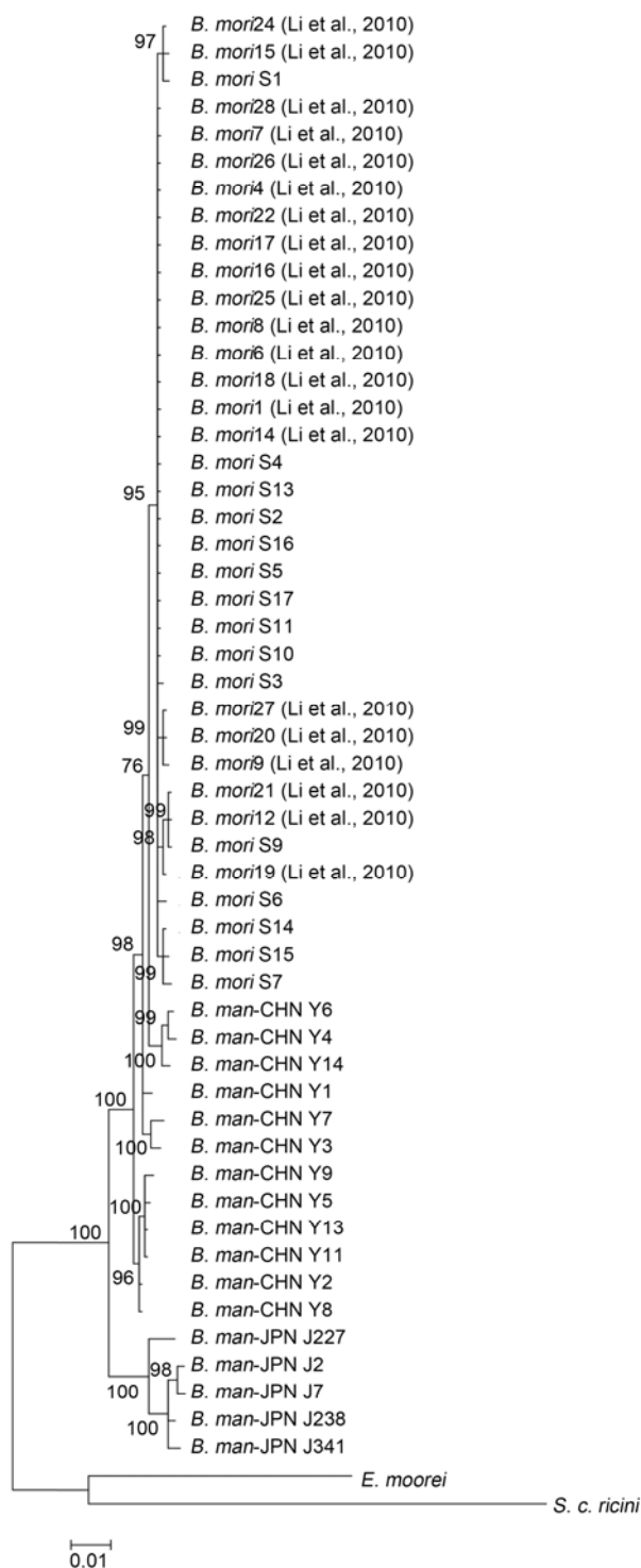
Appendix Figure 2 Maximum likelihood tree based on the concatenated mtDNA. Support values above the branches represent ML bootstrap (left) and MP bootstrap values, and below the branches represent Bayesian posterior probabilities. “—” indicates bootstrap values or BPP less than 50. B. man -CHN represents the Chinese wild silkworm; B. man -JPN represents Japanese wild silkworm. Li et al., 2010 refers to sequences obtained from Li et al., 2010 [8].
