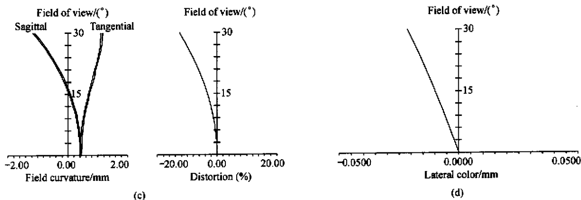
Fig. 2. Hybrid refractive-diffractive eyepiece. (a) Two dimensional layout; (b) transverse ray fan aberration; (c) field curvature and distortion; (d) lateral color aberration.
