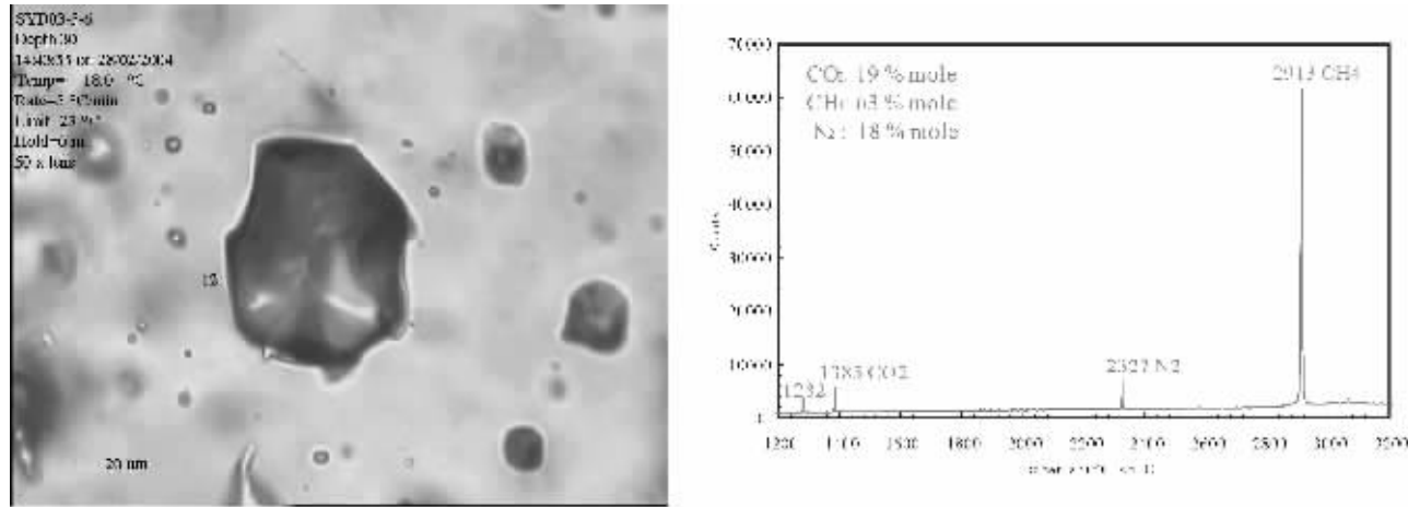
图 7 气相 \text{CH}_4\text{-N}_2\text{-CO}_2(\text{V}_{\text{CH}_4+\text{N}_2+\text{CO}_2}) 包裹体及激光拉曼光谱 Fig.7 Gas \text{CH}_4\text{-N}_2\text{-CO}_2(\text{V}_{\text{CH}_4+\text{N}_2+\text{CO}_2}) inclusions and laser Raman spectra
