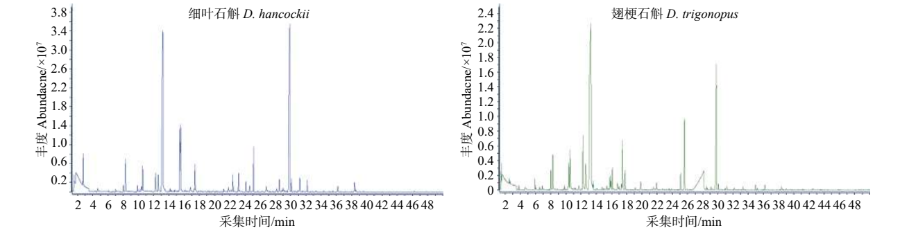
图 2 2 种浓香型石斛花挥发成分的总离子流图 Fig. 2 Ion chromatogram of volatile constituents in two Dendrobium species flower
