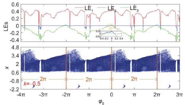
Figure 7 Memristor initial-value-related (top) LE spectra and (bottom) bifurcation diagram at fixed k = -0.5 , which demonstrate the infinite coexisting patterns boosted by the memristor initial value with fixed 2\pi offset.
