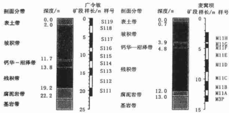
图 2 云南上芒岗金矿床红色粘土剖面分带 Fig. 2 Red clay profiles of the Shangmanggang gold deposit
