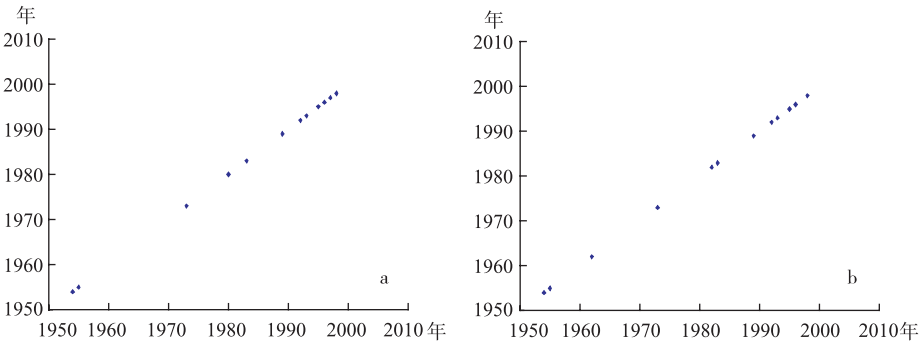
图 4 鄱阳湖区洪灾损失较大年份时间分布(a: 灾害总损失; b: 农田受灾面积) Fig.4 Time sequence of larger flood disaster loss in Lake Poyang region
