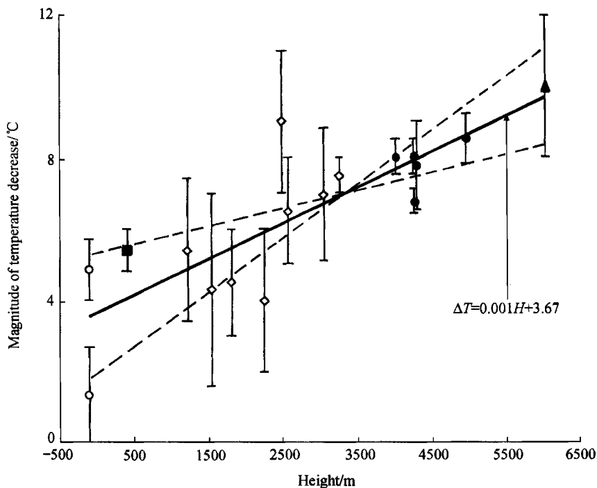
Fig. 2. The magnitudes of temperature decreases at different elevations in the equator during the LGM revealed by various kinds of methods. ○, Ocean data; ■, noble gas data; ◇, pollen data; ●, snow line data; ▲, ice core data.
