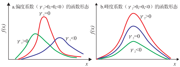
图 3 不同偏度系数和峰度系数的函数形态 Fig.3 Function forms of different coefficients of skewness and kurtosis
