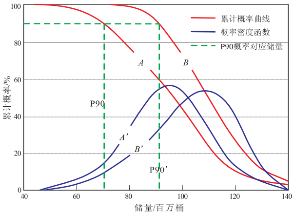
图 2 不同的概率密度函数及其对应的累计概率曲线 Fig.2 Different probability density functions and corresponding cumulative probability curves
