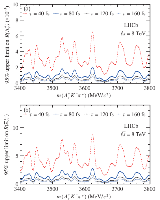
Figure 5 (Color online) Upper limits on (a) \mathcal{R}(\Lambda_c^+) and (b) \mathcal{R}(\Xi_{cc}^{++}) at 95% credibility level as a function of m(\Lambda_c^+ K^- \pi^+) at \sqrt{s} = 8 \text{ TeV} for four \Xi_{cc}^{++} lifetime hypotheses.
