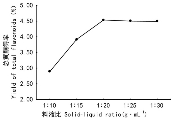
图 4 料液比对黑老虎叶总黄酮得率的影响 Fig. 4 Effects of solid-liquid ratio on yield of total flavonoids from Kadsura coccinea leaves
