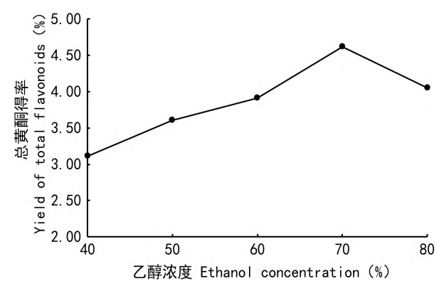
图 2 乙醇浓度对黑老虎叶总黄酮得率的影响 Fig. 2 Effects of ethanol concentration on yield of total flavonoids from Kadsura coccinea leaves
