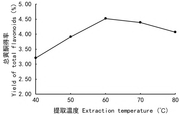
图 3 提取温度对黑老虎叶总黄酮得率的影响 Fig. 3 Effects of extraction temperature on yield of total flavonoids from Kadsura coccinea leaves
