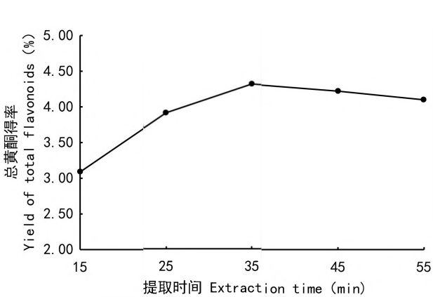
图 1 提取时间对黑老虎叶总黄酮得率的影响 Fig. 1 Effects of extraction time on yield of total flavonoids from Kadsura coccinea leaves
