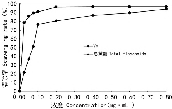
图 5 黑老虎叶总黄酮对 DPPH 清除能力 Fig. 5 Scavenging ability on DPPH of total flavonoids from Kadsura coccinea leaves
