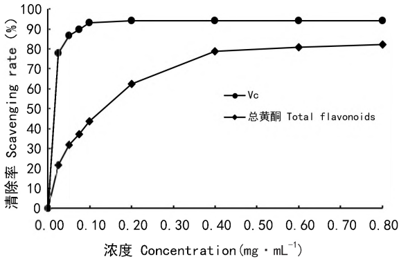
图 6 黑老虎叶总黄酮对 ·OH 清除能力 Fig. 6 Scavenging ability on ·OH of total flavonoids from Kadsura coccinea leaves
