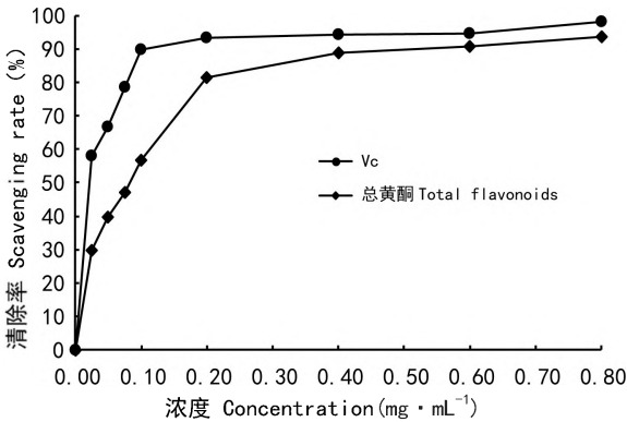
图 7 黑老虎叶总黄酮对超氧阴离子清除能力 Fig. 7 Scavenging ability on superoxide anion of total flavonoids from Kadsura coccinea leaves
