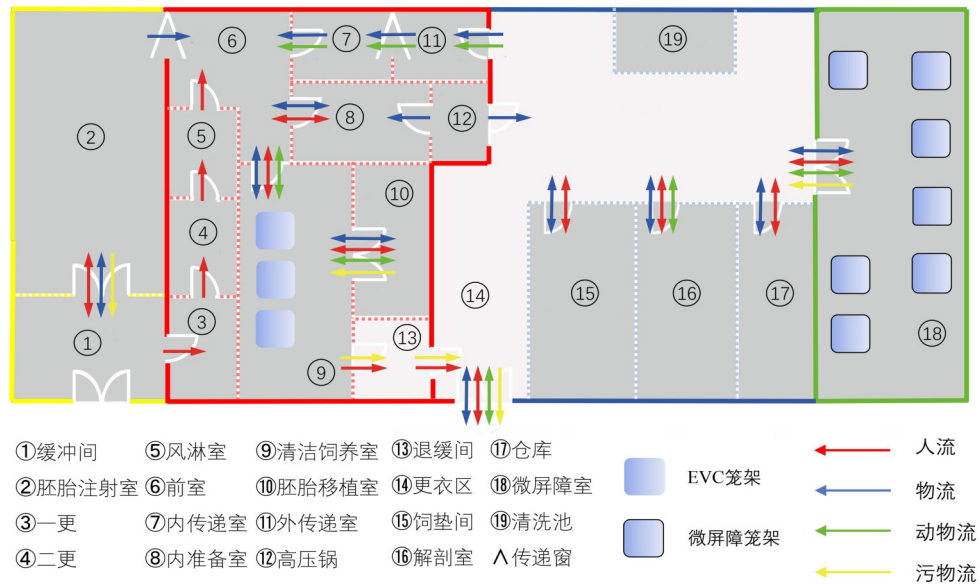
图1 设施平面图 Figure 1 Facility floor plan
