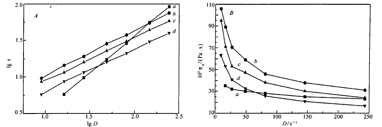
图 1 不同有机硅用量的乳液流变曲线 Fig. 1 Rheological curves of silicone-acrylate emulsion with different Si-1 contents. \omega(\text{Si-1})/\% : a. 0; b. 8; c. 18; d. 24 Si-1: acryloyl-propyl-tri-isopropyl silicone
