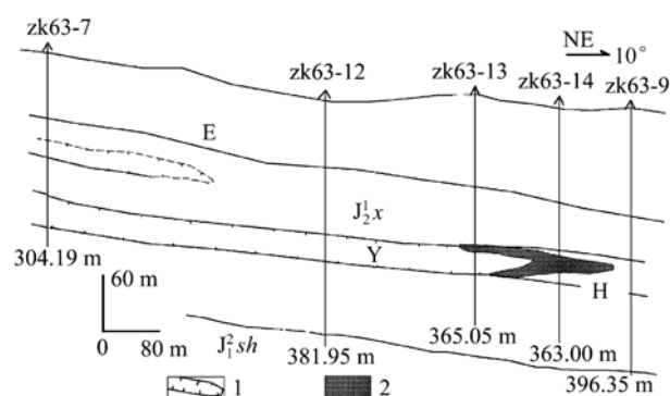
Fig. 3. Development characteristics of uranium orebodies under the control of No. 63 exploration line. 1, Interlayered oxidation zone; 2, uranium deposits (redox zone). Y, Oxidation zone; H, reduction zone; E, Tertiary.
