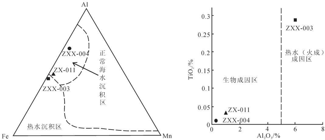
图 2 香山群硅质岩 Fe-Mn-Al 三元图解和 \text{Al}_2\text{O}_3 - \text{TiO}_2 图解 Fig.2 Fe-Mn-Al and \text{Al}_2\text{O}_3 - \text{TiO}_2 diagrams of cherts in the Xiangshan Group
