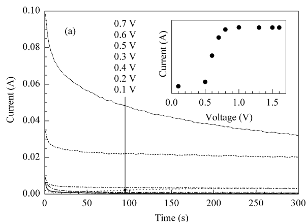
Figure 5. (a) Amperometric i-t curves during the electrolysis of ammonia processes in 2 mol/L \text{NH}_3 /1 mol/L KOH solution at 25 °C obtained at different applied potentials. The inset shows plot of the current as a function of applied potential in the electrolytic cell; (b) Galvanostatic curve obtained at a current density of 5 mA/cm 2 at 25 °C in the electrolytic cell filled with 2 mol/L \text{NH}_3 /5 mol/L KOH solution. The inset presents the galvanostatic response in an electrolytic cell filled with 5 mol/L KOH aqueous solution using the same electrodes
