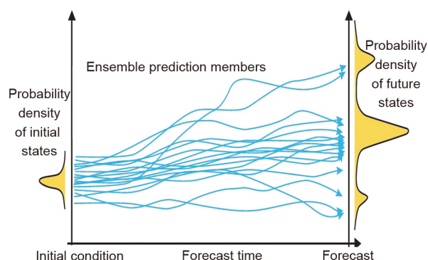
Figure 3 The framework of ensemble prediction (from http://old.ecmwf.int/about/corporate_brochure/leaflets/EPS-2012.pdf ).
