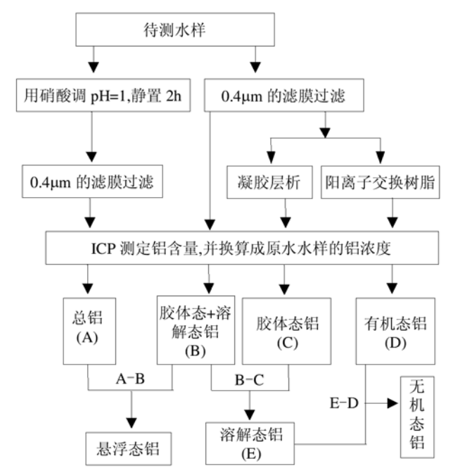
图 1 铝形态的分析流程及各铝形态间的关系 Fig.1 Procedure for analyzing aluminum species and relationship between aluminum species
