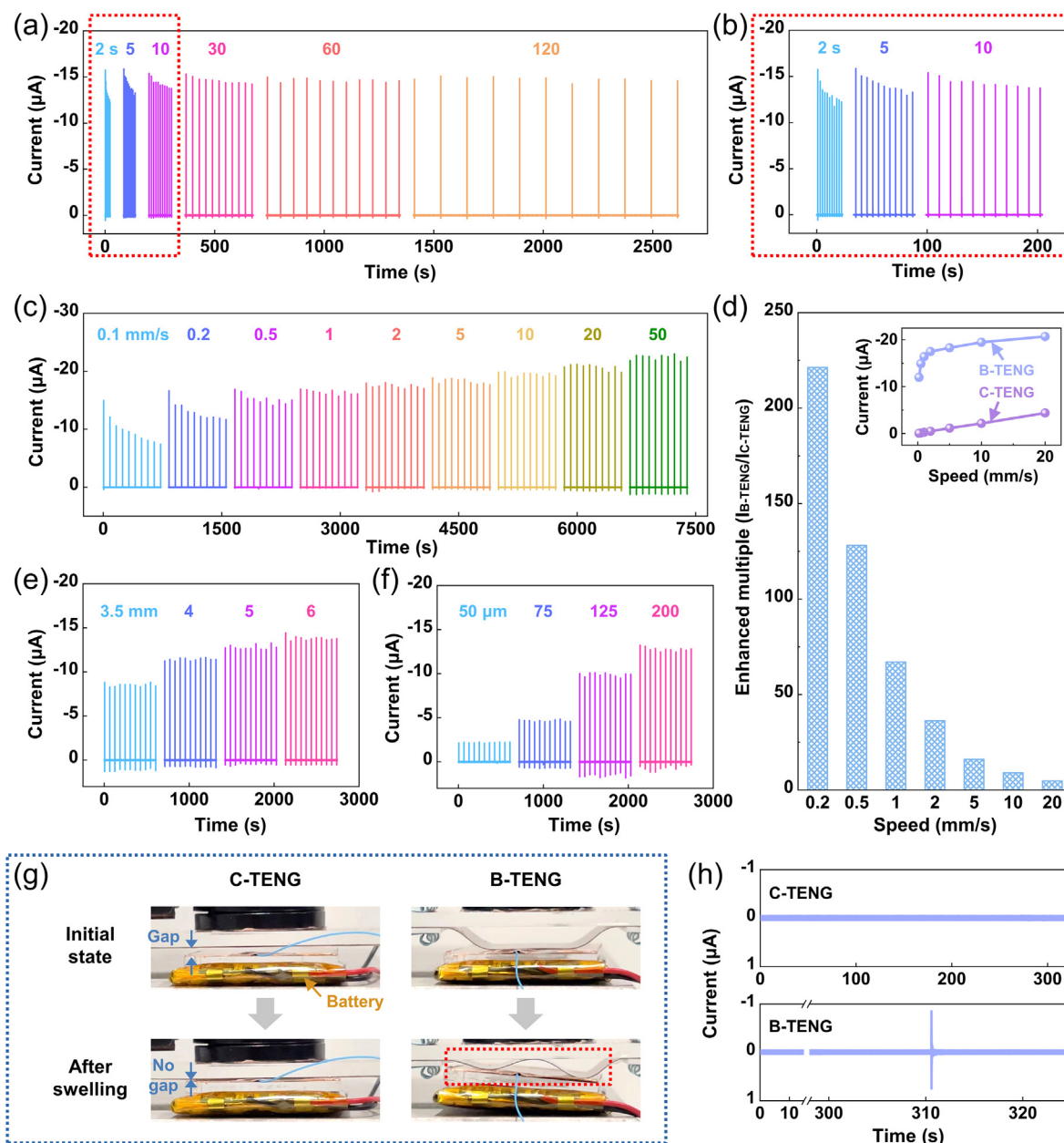
Fig. 2. Effect of different parameters on B-TENG current and monitoring of LIB swelling. (a, b) Current of B-TENG at different interval times. (c) B-TENG current at speeds from 0.1 to 50 \text{mm s}^{-1} when the time interval is 80 s. (d) Current enhancement of B-TENG relative to C-TENG at different speeds. The inset is comparison of current between B-TENG and C-TENG at different speeds. (e) Current of B-TENG at different heights. (f) Current of B-TENG at different thicknesses. (g) Physical diagrams and (h) currents of C-TENG and B-TENG monitoring of LIB swelling.
