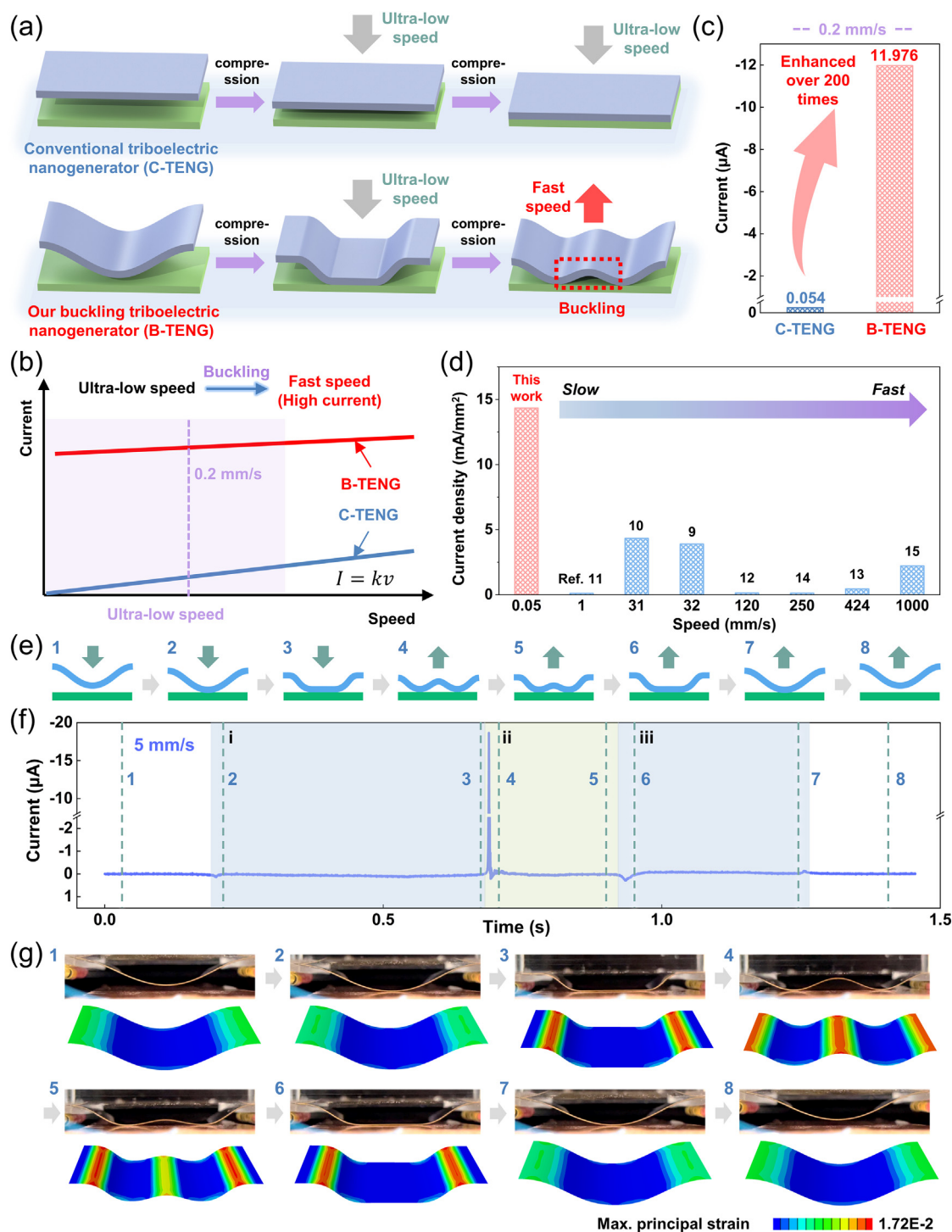
Fig. 1. Working mechanism and superiority of B-TENG. (a) Contact behavior of C-TENG and B-TENG at ultra-low speed. (b) Schematic of current output with respect to speed for C-TENG and B-TENG. (c) Comparison of current output of B-TENG and C-TENG at ultra-low speed of 0.2 \text{ mm s}^{-1} . (d) Comparison of current density at minimum speed of B-TENG with different TENGs. (e) Deformation states of B-TENG under a complete motion period. (f) Current waveform of B-TENG and (g) physical diagram of the curved structure and the corresponding strain distribution of polyimide under a complete motion period at 5 \text{ mm s}^{-1} .
