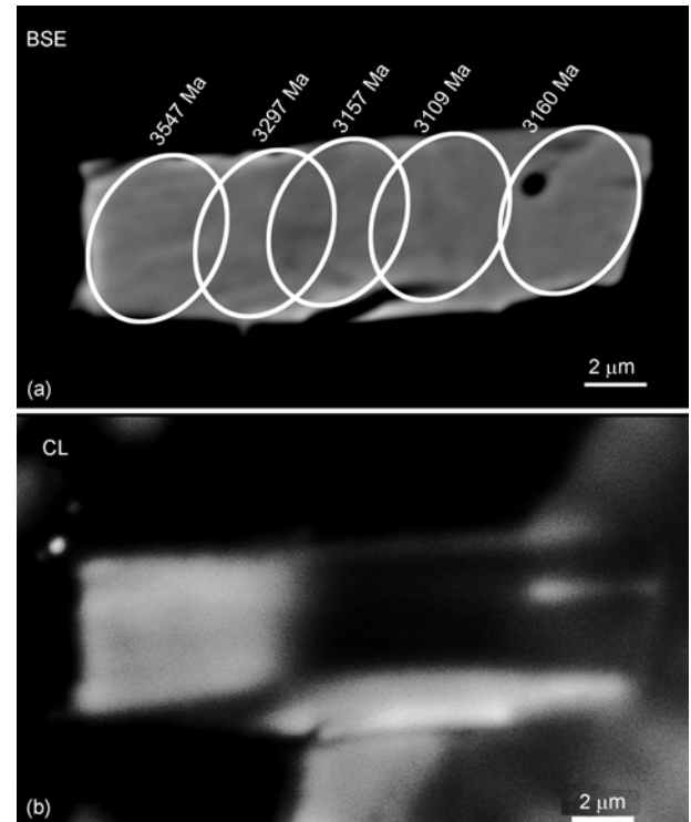
Figure 5 Back-scattered electron (BSE) (a) and CL (b) images of a baddeleyite grain in LAP 02224. The ellipsoidal circles indicate the SIMS spot locations. Bright areas in the CL image are older than darker areas.
