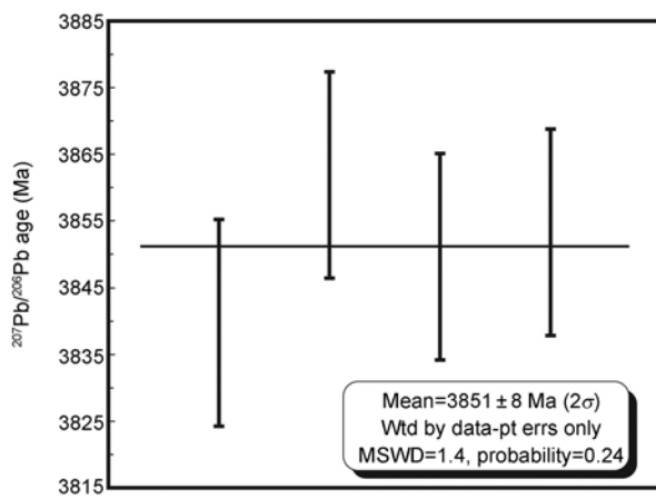
Figure 4 Weighted mean ^{207}\text{Pb}/^{206}\text{Pb} age of zirconolite in MIL 05035.
