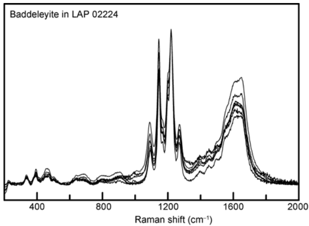
Figure 3 Raman spectra (200–2000 \text{cm}^{-1} ) of baddeleyite in LAP 02224.
