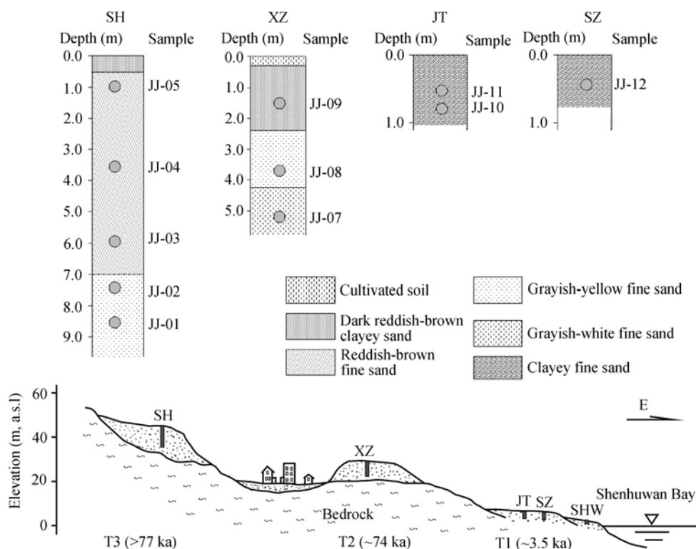
Figure 2 Sketch map showing the three marine terraces in Jinjiang, Fujian Province, China, and the sections for OSL sampling. XZ, Xiangzhi section; SHW, Shenhuan section; SH, Shenhuan section; JT, Jintiancun section; SZ, Shizhencun section.
