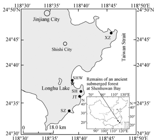
Figure 1 Location map showing the study area and the section sites for OSL sampling. XZ: Xiangzhi section, SHW: Shenhuiwan section, SH: Shenhui section, JT: Jintiancun section, SZ: Shizhencun section.
