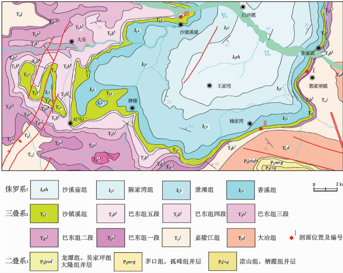
图 3 秭归盆地三叠系分布及剖面位置图 Fig.3 Distribution of the Triassic strata and sections in THE Zhiguai basin
