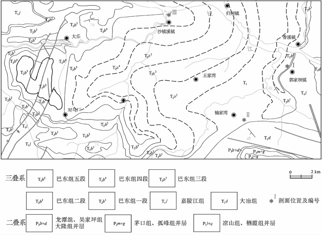
图 4 秭归盆地巴东组底图 Fig.4 Base map of the Badong Formation in the Zigui basin
