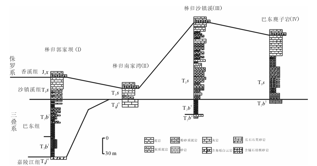
图 2 秭归盆地三叠系巴东组、沙镇溪组沉积柱状对比图 T 1j —下三叠统嘉陵江组;T 2b 1 —T 2b 5 —中三叠统巴东组一段—五段;T 3s —上三叠统沙镇溪组;J 1x —下侏罗统香溪组 Fig.2 Columns of the Triassic Badong and Shazhenxi formations in the Zigui basin T 1j —Lower Triassic Jialingjiang Formation;T 2b 1 —T 2b 5 —The first to fifth members of the Middle Triassic Badong Formation;T 3s —Upper Triassic Shazhenxi Formation;J 1x —Lower Jurassic Xiangxi Formation
