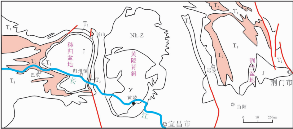
图 1 中三叠统巴东组、上三叠统沙镇溪组分布 γ—花岗岩类;Nh—Z—南华系—震旦系;T 1 —下三叠统;T 2 —中三叠统;T 3 —上三叠统;J—侏罗系 Fig.1 Distribution of the Middle Triassic Badong and Upper Triassic Shazhenxi formations γ—Granite;Nh—Z—Nanhuaian—Sinian;T 1 —Lower Triassic;T 2 —Middle Triassic;T 3 —Upper Triassic;J—Jurassic
